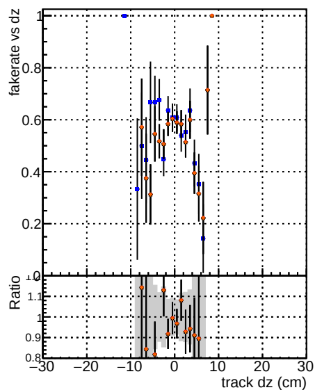
Fake rate vs dz Legend: DOM, GKE, TThor, DOM MKL, TThorPU-updated, DOM MKLPU-updated, New PLBNN-2
