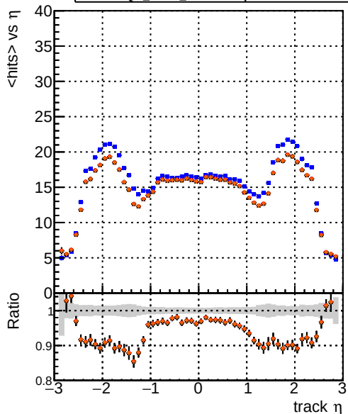
Legend: DQM_CKF_TTbar (blue line), DQM_mkFit_TTbarPU-updated (red line), DQM_mkFit_TTbarPU-updated-newPLDNN (black line), DQM_mkFit_TTbarPU-updated-newPLDNN-2 (orange line) mean hit
