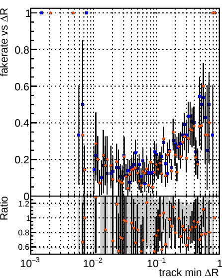
Fake rate vs \Delta R (track, jet) for DOM, CKE, Ttbar, mkrfit, TtbarPU-updated, and PLBNN-2
