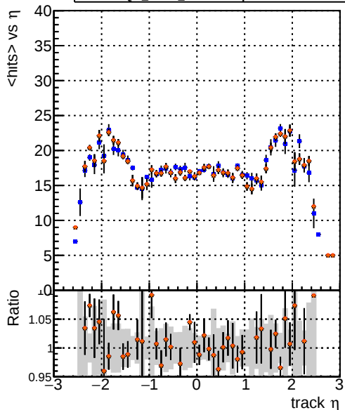
— DQM_CKF_TTbar — DQM_mkFit_TTbarPU-updated — DQM_mkFit_TTbarPU-updated-newPLDNN — DQM_mkFit_TTbarPU-updated-newPLDNN-2 mean hit
