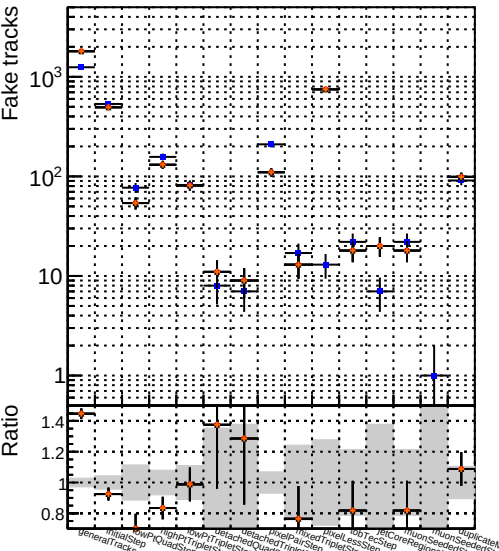
Number Model 1 DQM_mkFit_TTbarPU-updated 2 DQM_mkFit_TTbarPU-updated-newPLDNN 3 DQM_mkFit_TTbarPU-updated-newPLDNN-2
