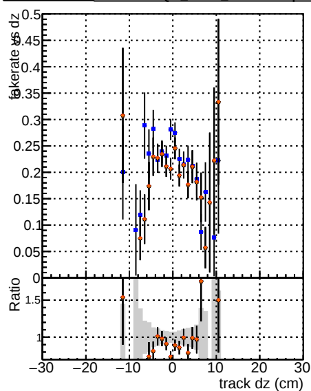
Legend for Fake rate vs d, Duplicates Rate vs Dxy, and Pileup rate vs dxy plots: — DOM GKE TThor — DOM MKEL TThor — DOM MKEL TThorPU-Updated-Res — DOM MKEL TThorPU-Updated-Res+PLDNN-2
