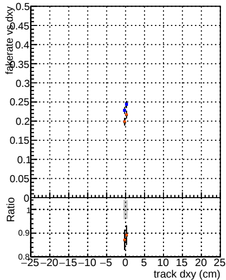
Legend for Fake rate vs d, Duplicates Rate vs Dxy, and Pileup rate vs dxy plots: — DOM GKE TThor — DOM MKEL TThor — DOM MKEL TThorPU-Updated-Res — DOM MKEL TThorPU-Updated-Res+PLDNN-2
