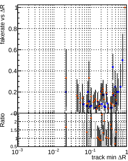
Fake rate vs \Delta R(\text{track, jet}) DOM CKE Ttbar PU-updated DOM mktfit Ttbar PU-updated DOM mktfit Ttbar PU-updated-new PLBNN-2
