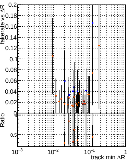
Fake rate vs \Delta R(\text{track}, \text{jet}) Legend: DOM (black), CKE (blue), Ttbar (red), PU-updated (orange), PU-updated-new (grey), PLBNN-2 (light blue)
