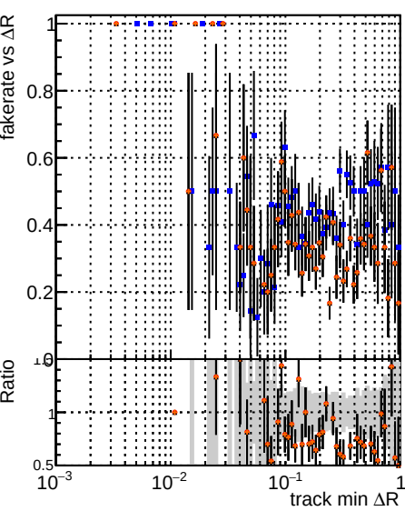
Fake rate vs \Delta R(\text{track, jet}) Legend: DOM (black), CKE (blue), TTbar (orange), PU-updated (red), PU-updated-new (grey), PLBNN-2 (dark grey)
