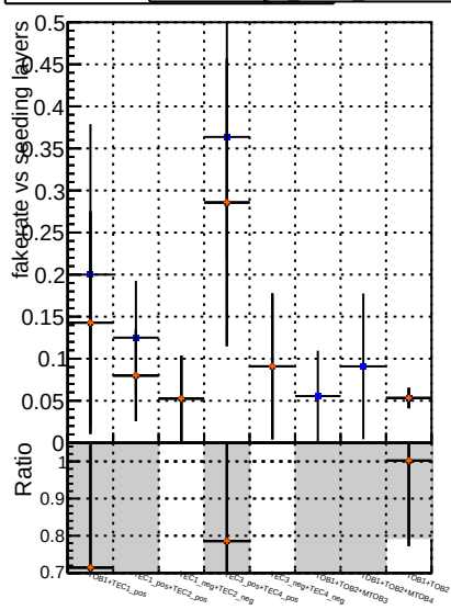
Fake rate vs. DOM SKI TThor DOM MREIL TThorPU-updated-raw DOM MREIL TThorPU-updated-raw+PLBNN-2
