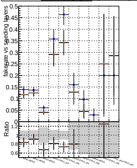
Fake rate vs. DOM GKE TTher TTher+BU-updated NewPLDNN.2
