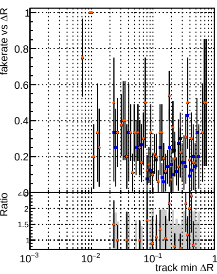
Fake rate vs \Delta R(\text{track, jet}) DOM CKE Ttbar PU-updated PU-updated-new PLBNN-2 DOM mktfit Ttbar PU-updated PU-updated-new PLBNN-2
