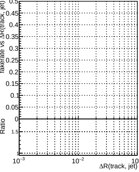
Fake rate vs \Delta R(\text{track, jet}) DOM CKE Ttbar PU-updated PU-updated-new PLBNN-2 DOM mktfit Ttbar PU-updated PU-updated-new PLBNN-2
