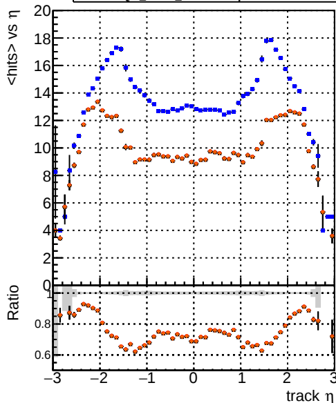
mean hit — DQM_CKF_TTbar — DQM_mkFit_TTbarPU-updated — DQM_mkFit_TTbarPU-updated-newPLDNN — DQM_mkFit_TTbarPU-updated-newPLDNN-2
