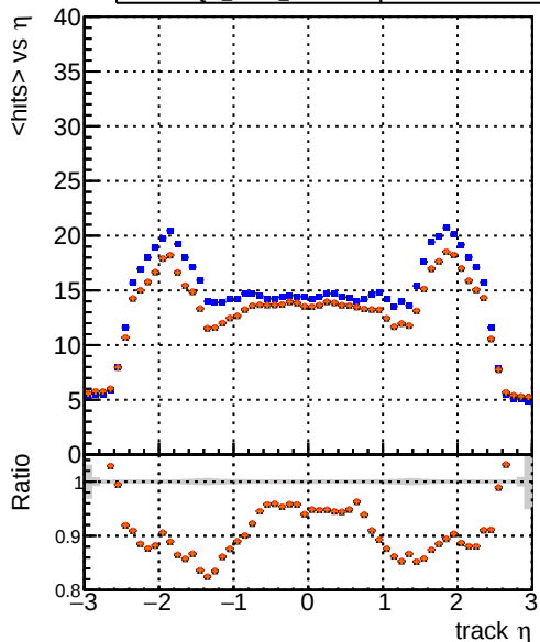
mean hit — DQM_CKF_TTbar — DQM_mkFit_TTbarPU-updated — DQM_mkFit_TTbarPU-updated-newPLDNN — DQM_mkFit_TTbarPU-updated-newPLDNN-2
