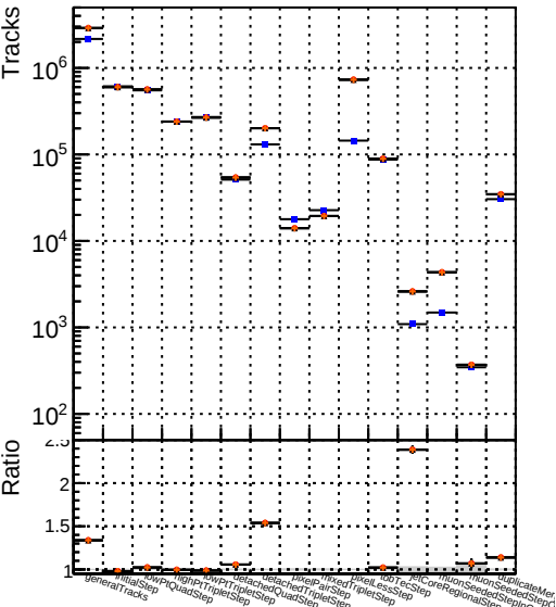
Number —■— DQM_CKF_TTbar —●— DQM_mkFit_TTbarPU-updated —▲— DQM_mkFit_TTbarPU-updated-newPLDNN —★— DQM_mkFit_TTbarPU-updated-newPLDNN-2
