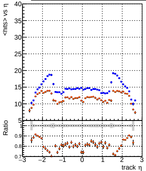
mean hit — DQM_CKF_TTbar — DQM_mkFit_TTbarPU-updated — DQM_mkFit_TTbarPU-updated-newPLDNN — DQM_mkFit_TTbarPU-updated-newPLDNN-2
