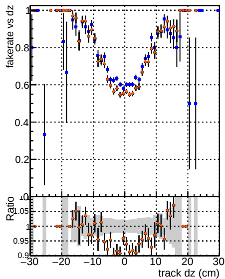
DOM GKE TThor TBarPU-updated-Res PLDNN-2 Fake rate vs d
