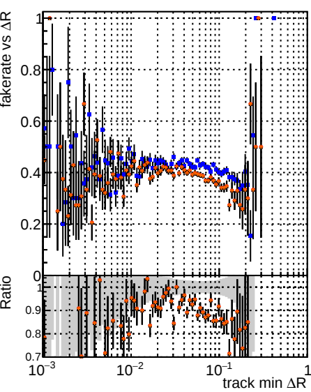
Fake rate vs \Delta R(\text{track, jet}) Legend: DOM (black), CKE (blue), Ttbar (orange), PU-updated (red), PU-updated-new (green), PLBNN-2 (purple)
