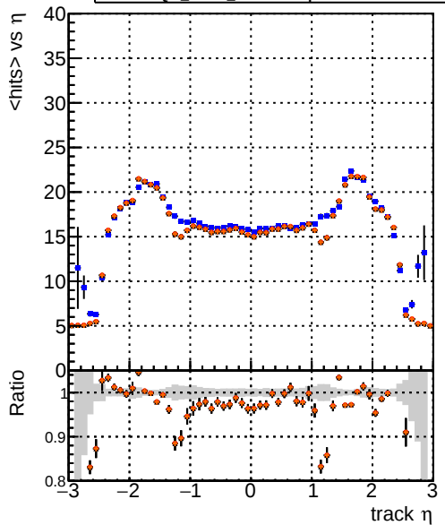
mean hit DQM_CKF_TTbar DQM_mkFit_TTbarPU-updated DQM_mkFit_TTbarPU-updated-newPLDNN-2 DQM_mkFit_TTbarPU-updated-newPLDNN-2
