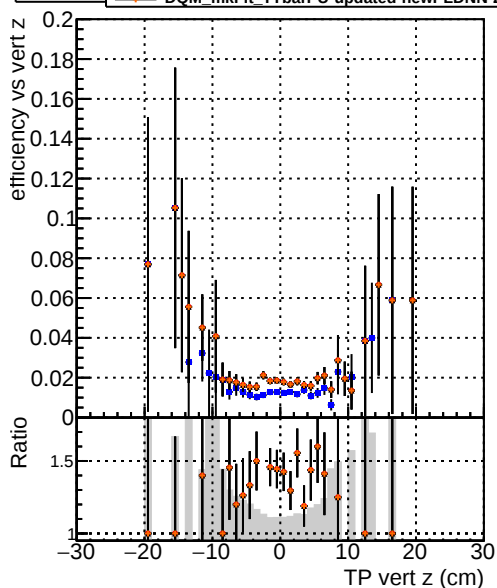
Efficiency vs vert z — DQM_CKF_TTbar — DQM_mkFit_TTbarPU-updated — DQM_mkFit_TTbarPU-updated-newPLDNN — DQM_mkFit_TTbarPU-updated-newPLDNN-2
