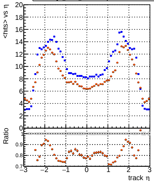
Legend: DQM_CKF_TTbar (blue), DQM_mkFit_TTbarPU-updated (red), DQM_mkFit_TTbarPU-updated-newPLDNN (black), DQM_mkFit_TTbarPU-updated-newPLDNN-2 (orange) mean hit
