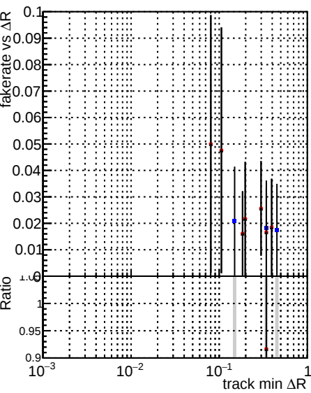
Legend: DOM_CKF_softQCD (blue dots), DOM_mkFit_SoftQCD-updated1 (red dots), DOM_mkFit_SoftQCD-updated1-newPLDNN (black dots)
