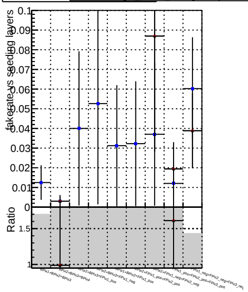
Fake rate vs. DOM CKF softOCB softOCB-updated1 DOM mktFit softOCB-updated1-newPLDNN
