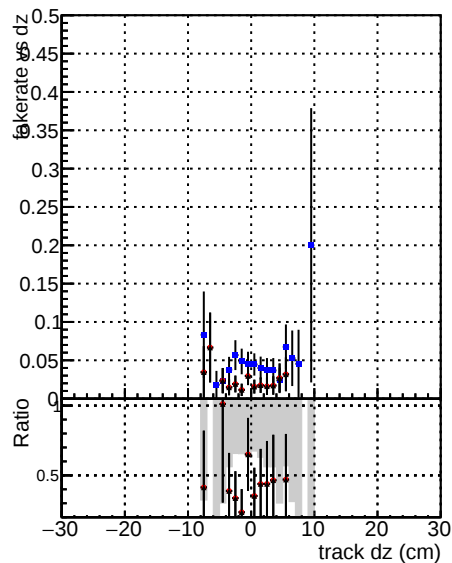
Fake rate vs dz —•— DOM CKF softOCB —•— DOM mktFit softOCB-updated1 —•— DOM mktFit softOCB-updated1-newPLDNN
