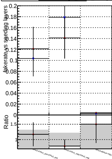
Fake rate vs. DOM CKF softOCB DOM CKF softOCB-updated1 DOM CKF softOCB-updated1-newPLDNN
