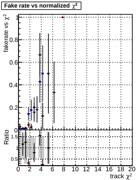
Fake rate vs. DOM CKF softOCB DOM CKF softOCB-updated1 DOM CKF softOCB-updated1-newPLDNN
