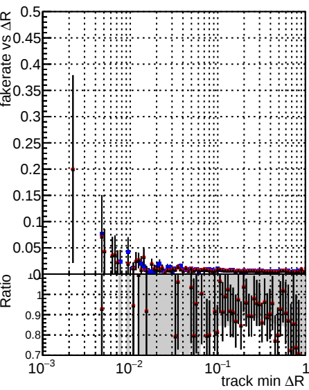
Legend: DQM_CKF_softQCD (black line), DQM_mkFit_SoftQCD-updated1 (red line), DQM_mkFit_SoftQCD-updated1-newPLDNN (blue line)
