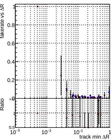
Legend: DQM_CKF_softQCD (blue circles), DQM_mkFit_SoftQCD-updated (red circles), DQM_mkFit_SoftQCD-DNNalliters (black circles)
