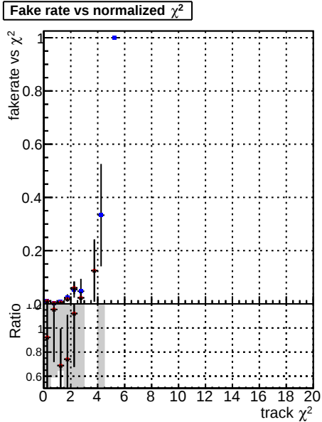
Fake rate vs. DOM CKF softOCB softOCB-updated DOM mktFit softOCB-BNNfilters
