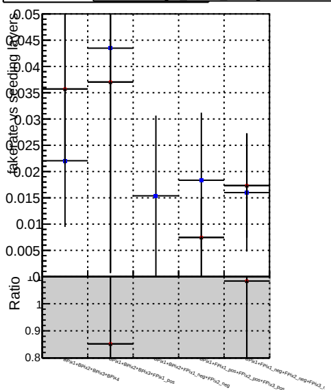
Fake rate vs. DOM CKF softOCB DOM mkrFit DOM mkrFit softOCB-DNNfilters
