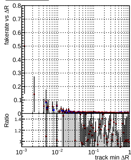
Legend: \square DOM_CKF_softQCD \square DOM_mkFit_SoftQCD-updated \square DOM_mkFit_SoftQCD-DNNalliters
