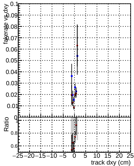
— DOM CKF softQCD — DOM CKF softQCD-updated — DOM mktFit softQCD-DNNfilters
