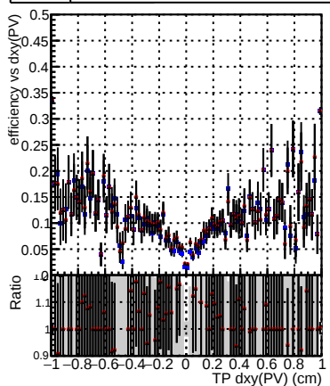
Efficiency DQM_n
