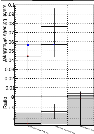
Fake rate vs. DOM CKF softOCB DOM mktFit softOCB-DNNfilters
