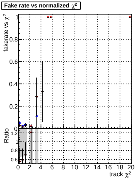
Fake rate vs. DOM CKF softOCB DOM mktFit softOCB-DNNfilters
