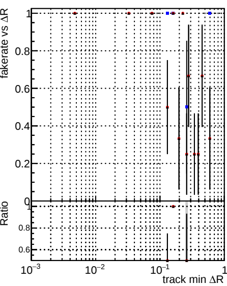
Fake rate vs ΔR(track, jet) Legend: DOM_CKF_softQCD (blue dots) DOM_mkFit_SoftQCD-updated (red dots) DOM_mkFit_SoftQCD-DNNalliters (black dots with error bars)
