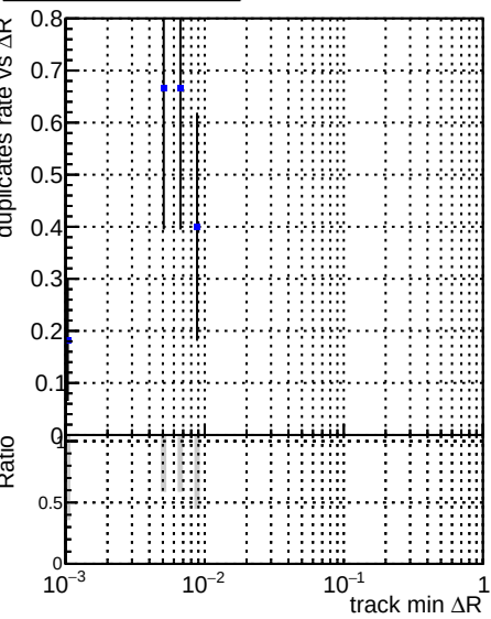
Legend: DQM_CKF_softQCD (blue dots), DQM_mkFit_SoftQCD-updated (red dots), DQM_mkFit_SoftQCD-DNNalliters (black dots)
