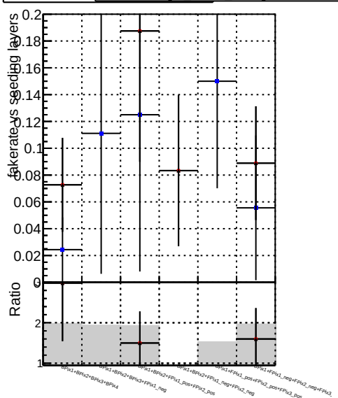
Fake rate vs. DOM CKF softOCB DOM CKF softOCB-updated DOM mktFit softOCB-DNNfilters
