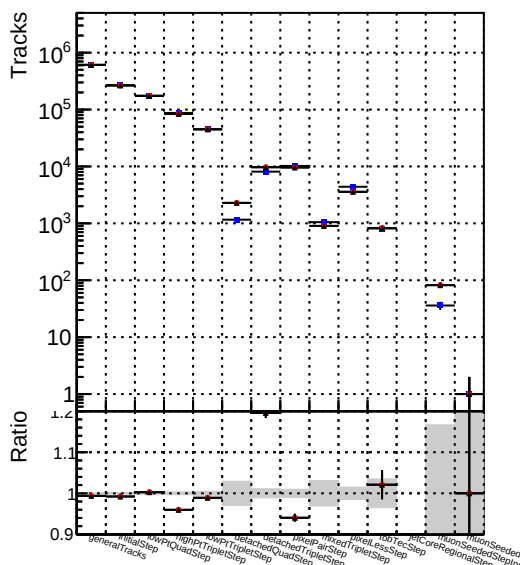
Number of tracks vs collection Legend: DQM_CKF_softQCD DQM_mkFit_SoftQCD-updated DQM_mkFit_SoftQCD-DNNalliters
