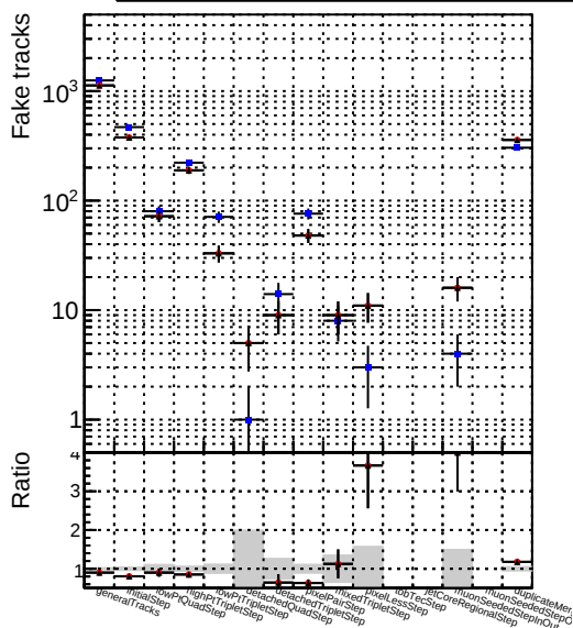
Number —●— DQM_mkFit_SoftQCD-updated —▲— DQM_mkFit_SoftQCD-DNNalliters
