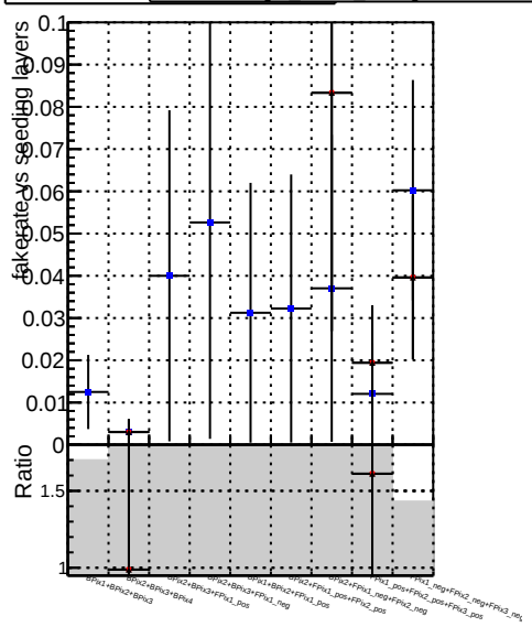
Fake rate vs. DOM CKF softOCB DOM-mkFit softOCB-updated DOM-mkFit softOCB-DNNfilters
