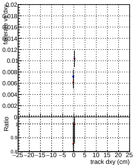
Legend for Fake rate vs dxy: DOM CKF softOCB DOM CKF softOCB-updated DOM mktFit softOCB-DNNfilters
