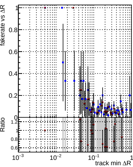
Legend: DOM_CKF_softQCD (blue squares), DOM_mkFit_SoftQCD-updated (red circles), DOM_mkFit_SoftQCD-DNNalliters (black crosses)
