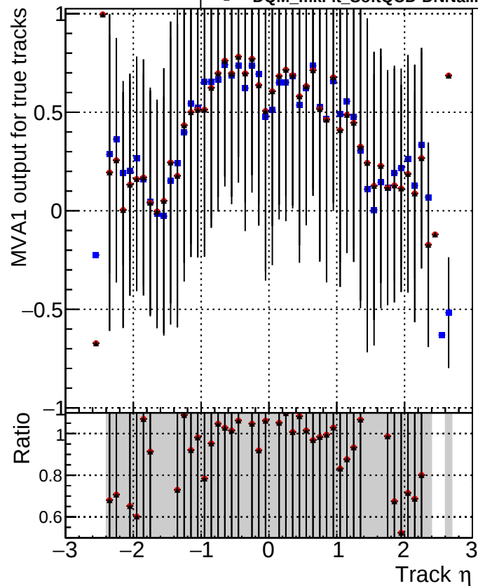
MVA1 of associated tracks (recoToSim) vs. track \eta Legend: DQM_CKF_softQCD (blue squares) DQM_mkFit_SoftQCD-updated (red circles) DQM_mkFit_SoftQCD-DNNalliters (black triangles)
