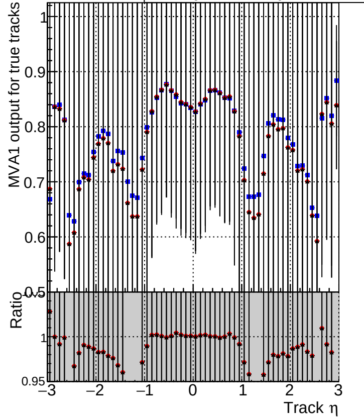
MVA1 of associated tracks (recoToSim) vs. track \eta Legend: ■ DQM_CKF_softQCD ● DQM_mkFit_SoftQCD-updated ▲ DQM_mkFit_SoftQCD-DNNalliters
