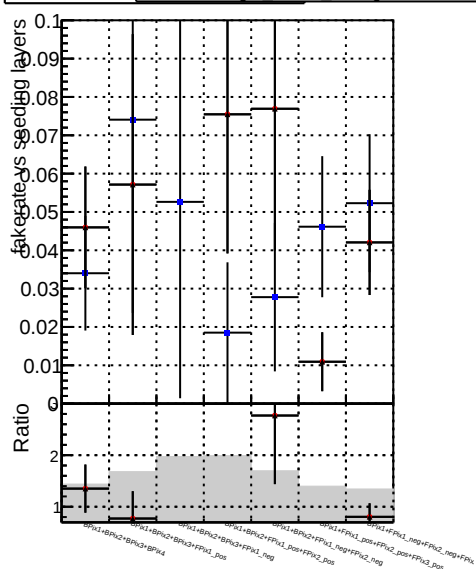
Fake rate vs. DOM CKF softOCB DOM CKF softOCB updated DOM mktFit softOCB-BNNvaliters
