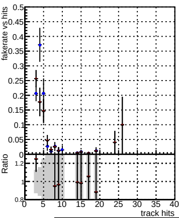
Fake rate vs hit Legend: DQM_CKF_softQCD (Blue dots) DQM_mkFit_SoftQCD-updated (Red dots) DQM_mkFit_SoftQCD-DNNalliters (Black dots)
