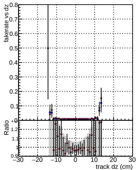
Fake rate vs dz DOM CKF softOCB DOM CKF softOCB-updated DOM mktFit softOCB-DNNfilters
