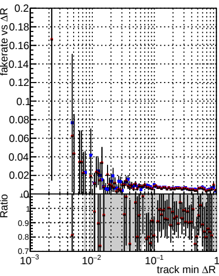
DOM_CKF_softQCD DOM_mkFit_SoftQCD-updated DOM_mkFit_SoftQCD-DNNalliters
