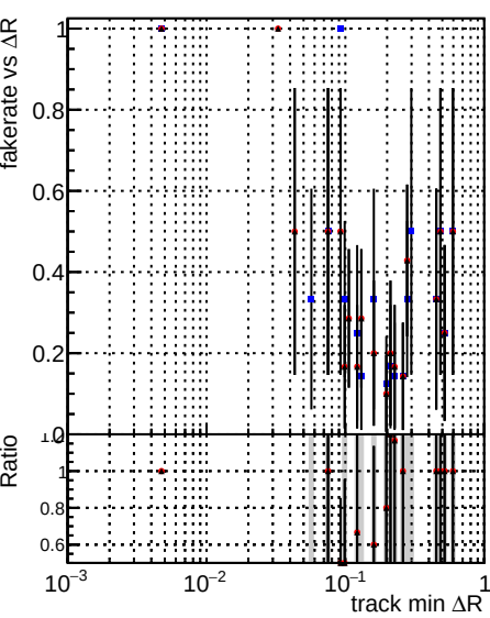
Fake rate vs \Delta R (track, jet) DOM_CKF_softQCD DOM_mkFit_SoftQCD-updated DOM_mkFit_SoftQCD-DNNalliters
