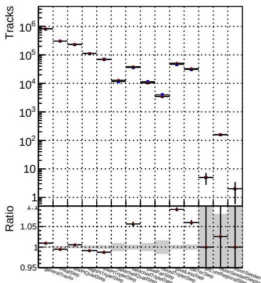
Number of tracks vs collection Legend: DQM_CKF_softQCD DQM_mkFit_SoftQCD-updated DQM_mkFit_SoftQCD-DNNsqcd100
